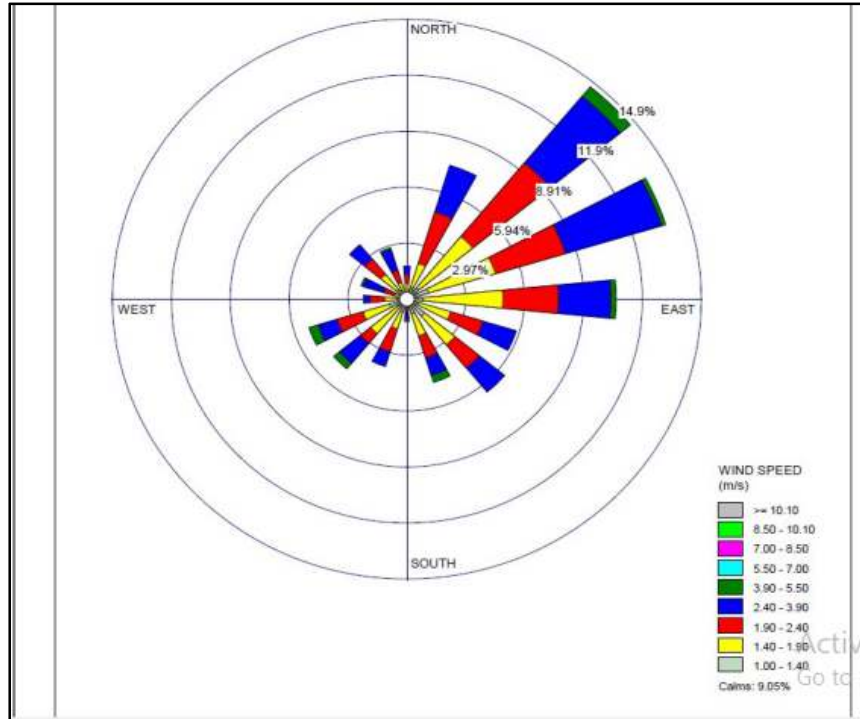
Figure 1: Wind Rose
